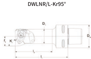
DWLNR/L-Kr95°
