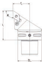
PDJNR/L-Kr 93°
