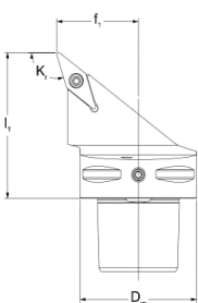
SVHBR/L-Kr 107.5°
