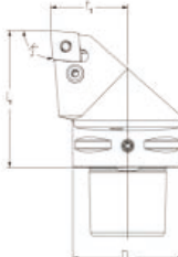
PCLNR/L-Kr 95°
