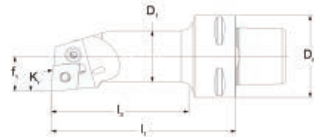
PCLNR/L-Kr95°
